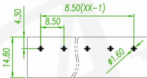
RECOMMENDED PCB LAOUT (PCB TOLERANCE ±0.05)
