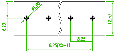
RECOMMENDED PCB LAOUT (PCB TOLERANCE ±0.05)
