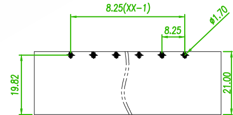
RECOMMENDED PCB LAOUT (PCB TOLERANCE ±0.05)
