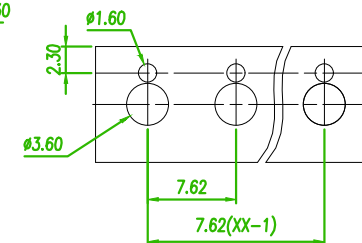
RECOMMENDED PCB LAOUT (PCB TOLERANCE ±0.05)
