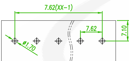
RECOMMENDED PCB LAOUT (PCB TOLERANCE ±0.05)
