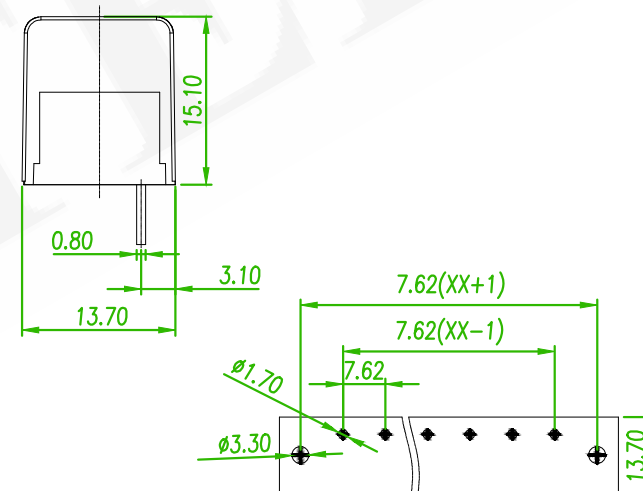
RECOMMENDED PCB LAOUT (PCB TOLERANCE ±0.05)
