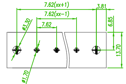
RECOMMENDED PCB LAOUT (PCB TOLERANCE ±0.05)
