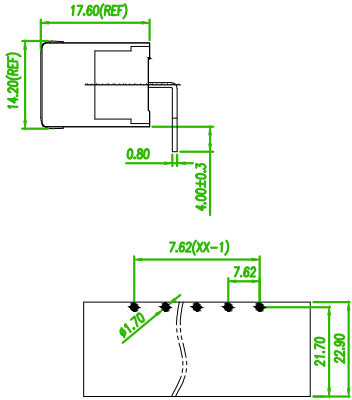
RECOMMENDED PCB LAOUT (PCB TOLERANCE ±0.05)
