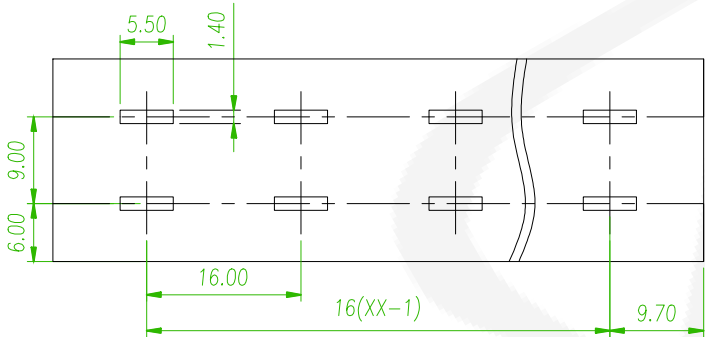
RECOMMENDED PCB LAYOUT (PCB TOLERANCE ±0.05)
