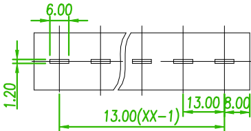
RECOMMENDED PCB LAOUT (PCB TOLERANCE ±0.05)
