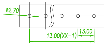
RECOMMENDED PCB LAOUT (PCB TOLERANCE ±0.05)
