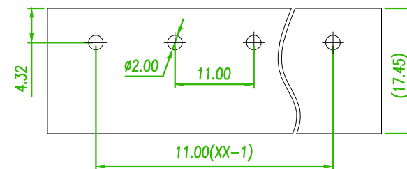
RECOMMENDED PCB LAOUT (PCB TOLERANCE ±0.05)
