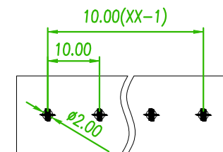
RECOMMENDED PCB LAOUT (PCB TOLERANCE ±0.05)
