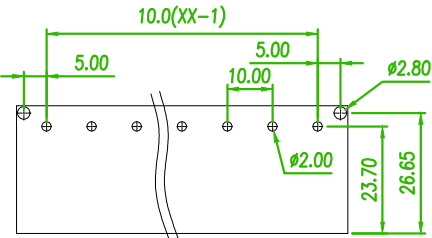
RECOMMENDED PCB LAOUT (PCB TOLERANCE ±0.05)
