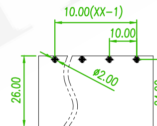
RECOMMENDED PCB LAOUT (PCB TOLERANCE ±0.05)
