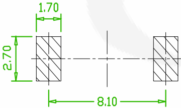
RECOMMENDED PCB LAYOUT (PCB TOLERANCE ±0.05)
