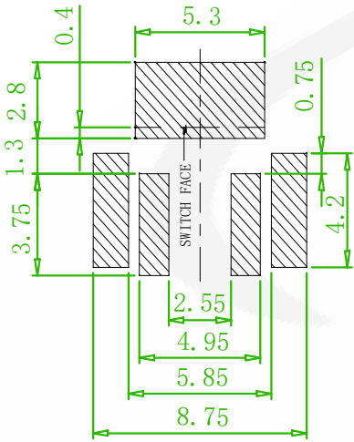
RECOMMENDED PCB LAYOUT (PCB TOLERANCE ±0.05)
