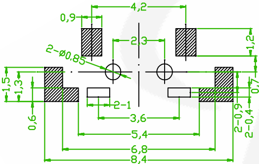
Top View Recommended PCB Layout (PCB TOLERANCE ±0.05)
