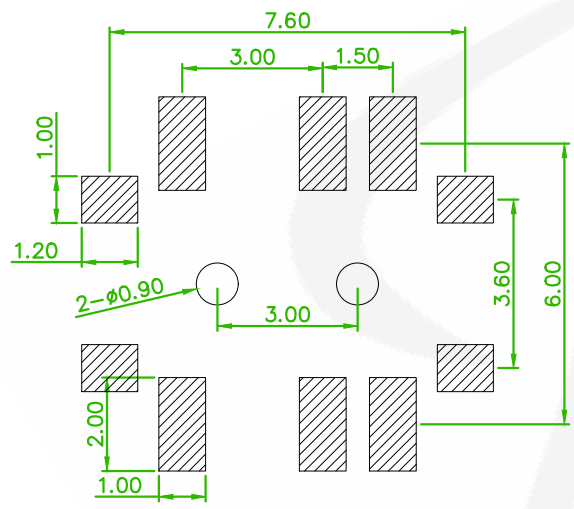
RECOMMENDED PCB LAYOUT (PCB TOLERANCE ±0.05)
