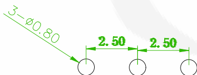
RECOMMENDED PCB LAYOUT (PCB TOLERANCE ±0.05)
