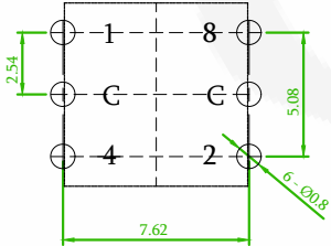
RECOMMENDED PCB LAOUT (PCB TOLERANCE ±0.05)
