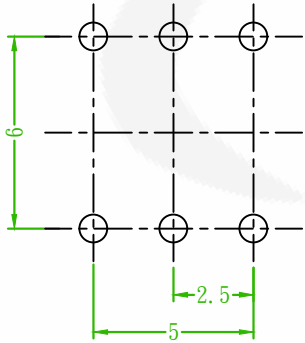
RECOMMENDED PCB LAYOUT (PCB TOLERANCE ±0.05)
