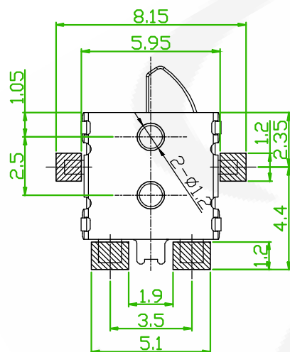
RECOMMENDED PCB LAYOUT (PCB TOLERANCE \pm 0.05 )
