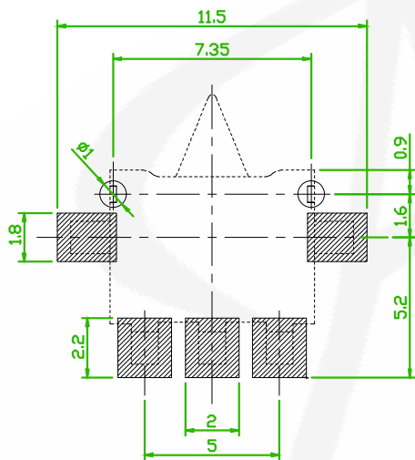
RECOMMENDED PCB LAYOUT (PCB TOLERANCE ±0.05)
