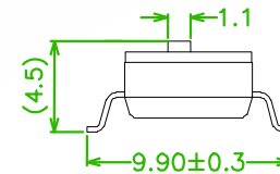
6SDMS01-045*** RAISED ACTUATOR TYPE
