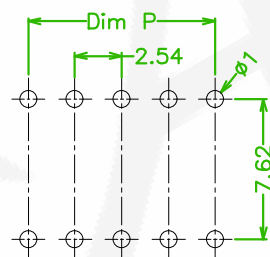
RECOMMENDED PCB LAYOUT (PCB TOLERANCE \pm 0.05 )
