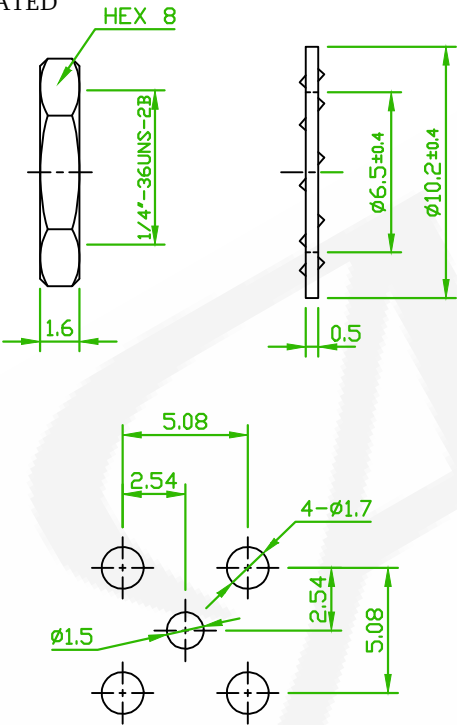
RECOMMENDED PCB LAYOUT (PCB TOLERANCE ±0.05)
