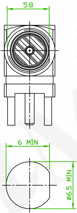
MOUNTING HOLES (REF)
