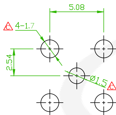
RECOMMENDED MOUNTING HOLES
