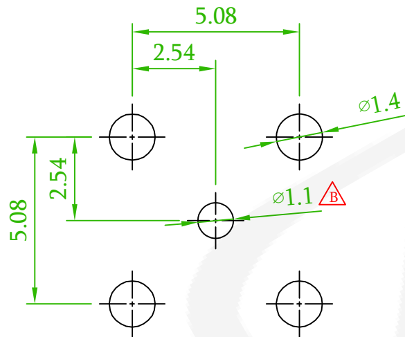
Recommended PCB Layout (PCB TOLERANCE \pm 0.1 )
