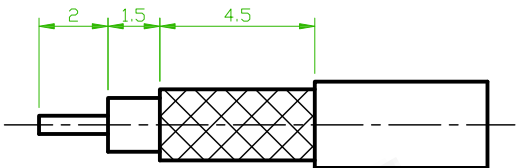
REFERENCE STRIP LENGTHS HEX Crimp Size : E
