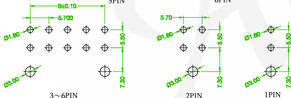
RECOMMENDED PCB LAYOUT (PCB TOLERANCE \pm 0.05 )
