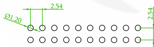
RECOMMENDED PCB LAYOUT (PCB TOLERANCE \pm 0.05 )
