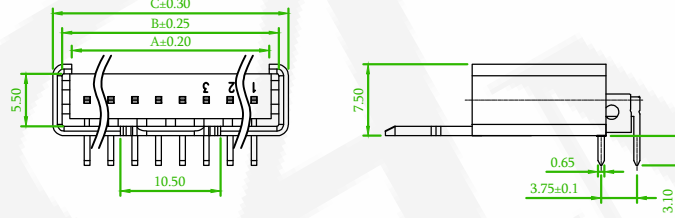
With Latch: 04-20 Pin
