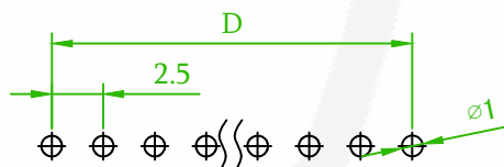
RECOMMENDED PCB LAYOUT (PCB TOLERANCE ±0.05)
