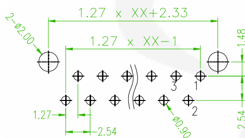
RECOMMENDED PCB LAYOUT (PCB TOLERANCE \pm 0.05 )
