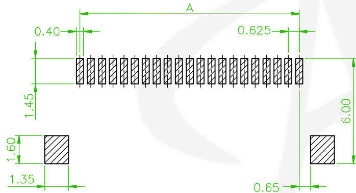
RECOMMENDED PCB LAYOUT (PCB TOLERANCE \pm 0.05 )
