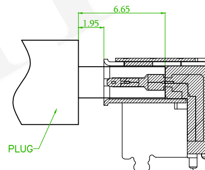
AFTER MATING
