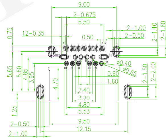
RECOMMENDED P.C.B LAYOUT(Both sides are sample)
