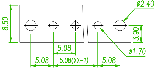
RECOMMENDED PCB LAOUT (PCB TOLERANCE ±0.05)
