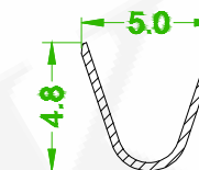
SECTION A-A CONDUCTOR CRIMP 12 AWG
