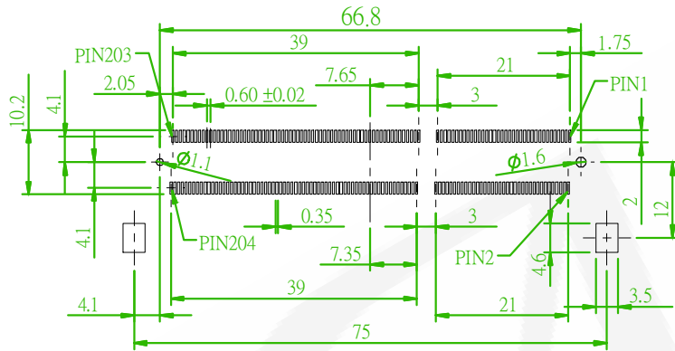
RECOMMENDED PCB LAYOUT (PCB TOLERANCE ±0.05)
