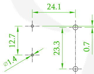
Recommended PCB Layout (PCB TOLERANCE \pm 0.1 )
