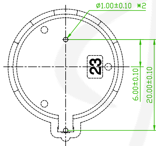
RECOMMEND PCB LAYOUT COMPONENT SIDE
