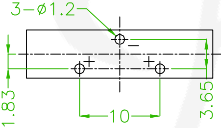
RECOMMENDED PCB LAYOUT (PCB TOLERANCE ±0.05)
