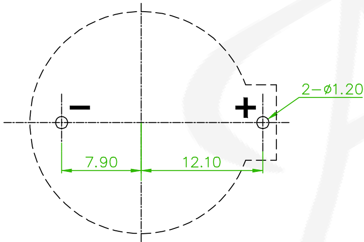
RECOMMENDED PCB LAYOUT (PCB TOLERANCE \pm 0.05 )
