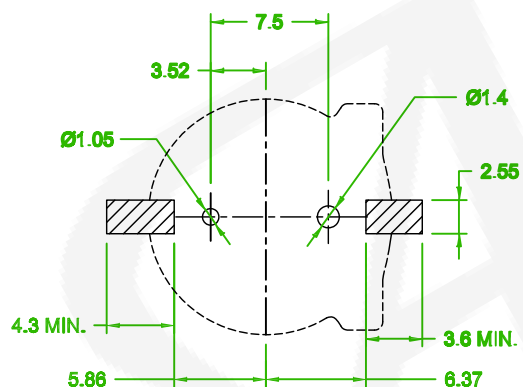
MOUNTING PAD & HOLE DETAIL
