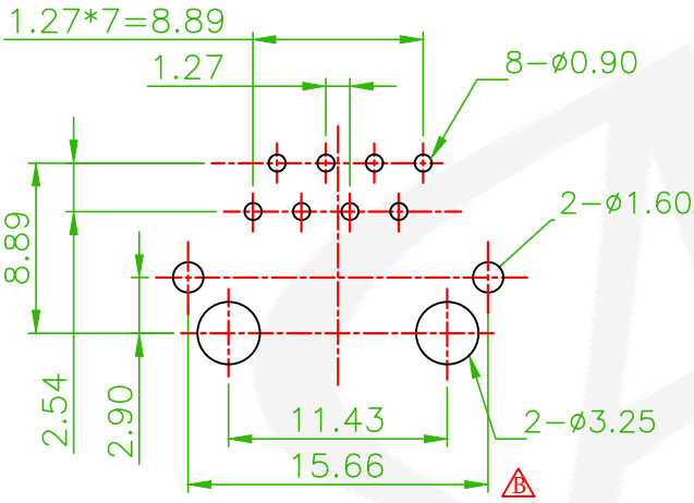
RECOMMENDED PCB LAYOUT (PCB TOLERANCE ±0.05)
