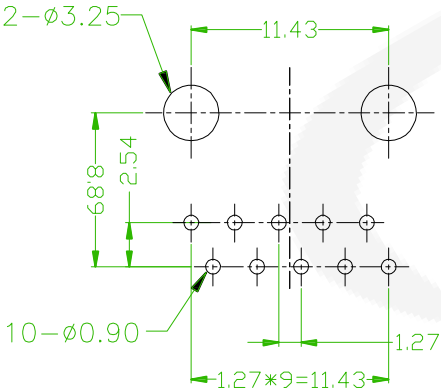
Recommended PCB Layout (PVB TOLERANCE±0.05)
