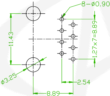
Recommended PCB Layout (Thickness=1.60mm) (PCB TOLERANCE ±0.05)
