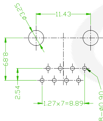
Recommended PCB Layout (PVB TOLERANCE±0.05)
